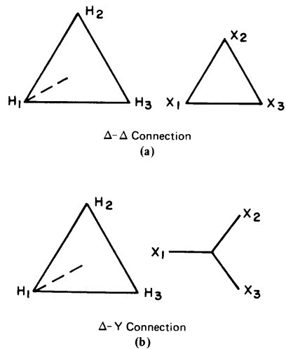
Figure 1— Angular Displacement
