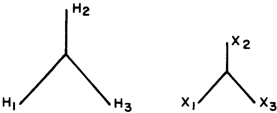
Figure 4— Y-Y Connection
